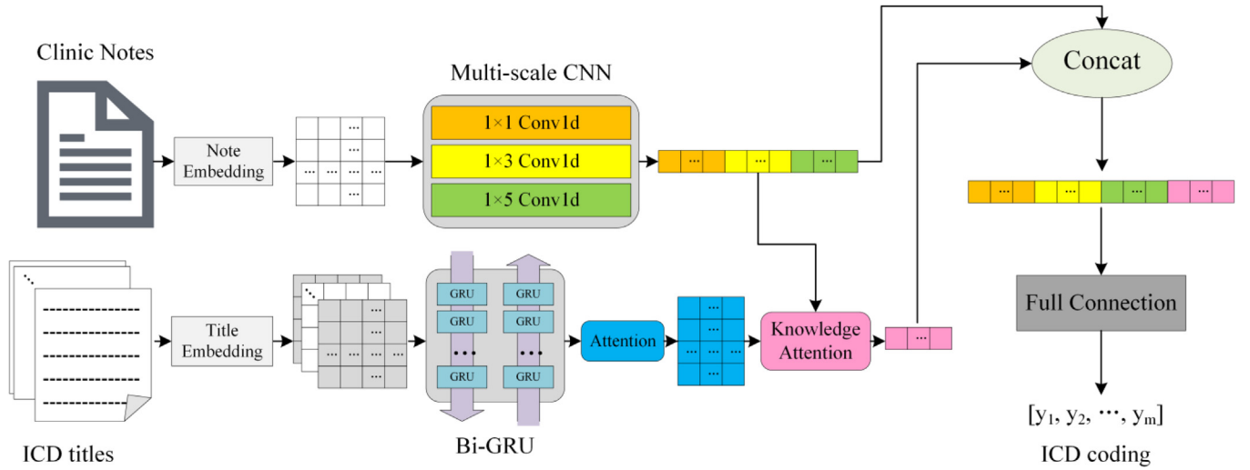
Fig. 1. The architecture of KAICD. KAICD has two inputs: a clinic note and all ICD titles. For a clinic note, KAICD uses a multi-scale CNN to extract its features. For all ICD titles, KAICD uses Attention-based Bidirectional Gated Recurrent Unit (Bi-GRU) to build a knowledge database. Depending on input clinic notes, the attention mechanism is applied to obtain knowledge vectors from the knowledge database. Finally, the features of clinic notes and the knowledge vectors are concatenated to predict the probability of ICD codes.
