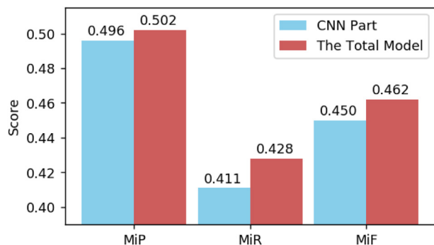
Fig. 4. Performances of the CNN part and the total model.
