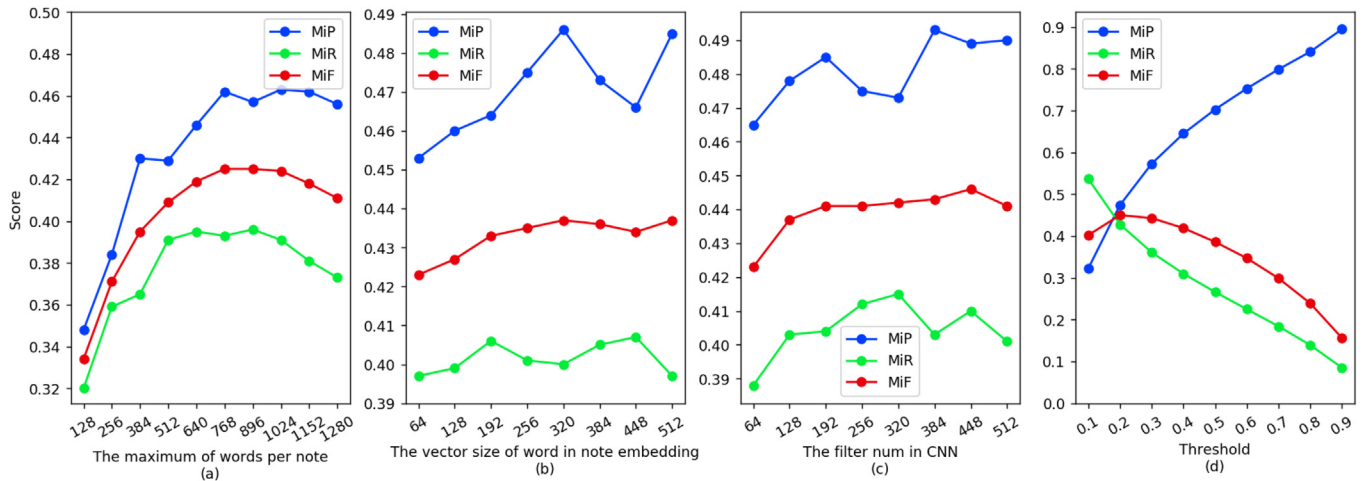
Fig. 3. Performances of our model in different parameters.
